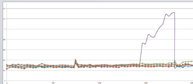
Six movers in online monitoring: the impending failure of a ball bearing shows several days in advance.
